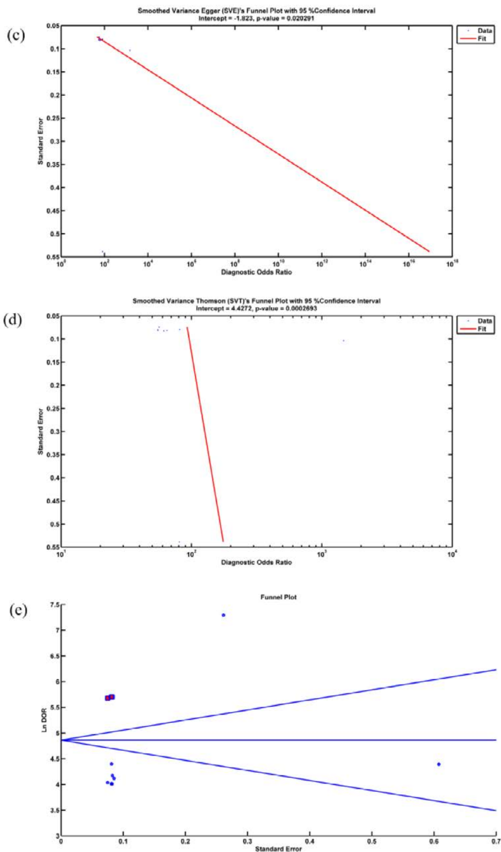
Figure 5. Publication bias test, (a) Egger's funnel plot (b) Deeks' funnel plot, (c) SVE funnel plot (d) SVT funnel plot, and (e) trim and fill assessment approach.
