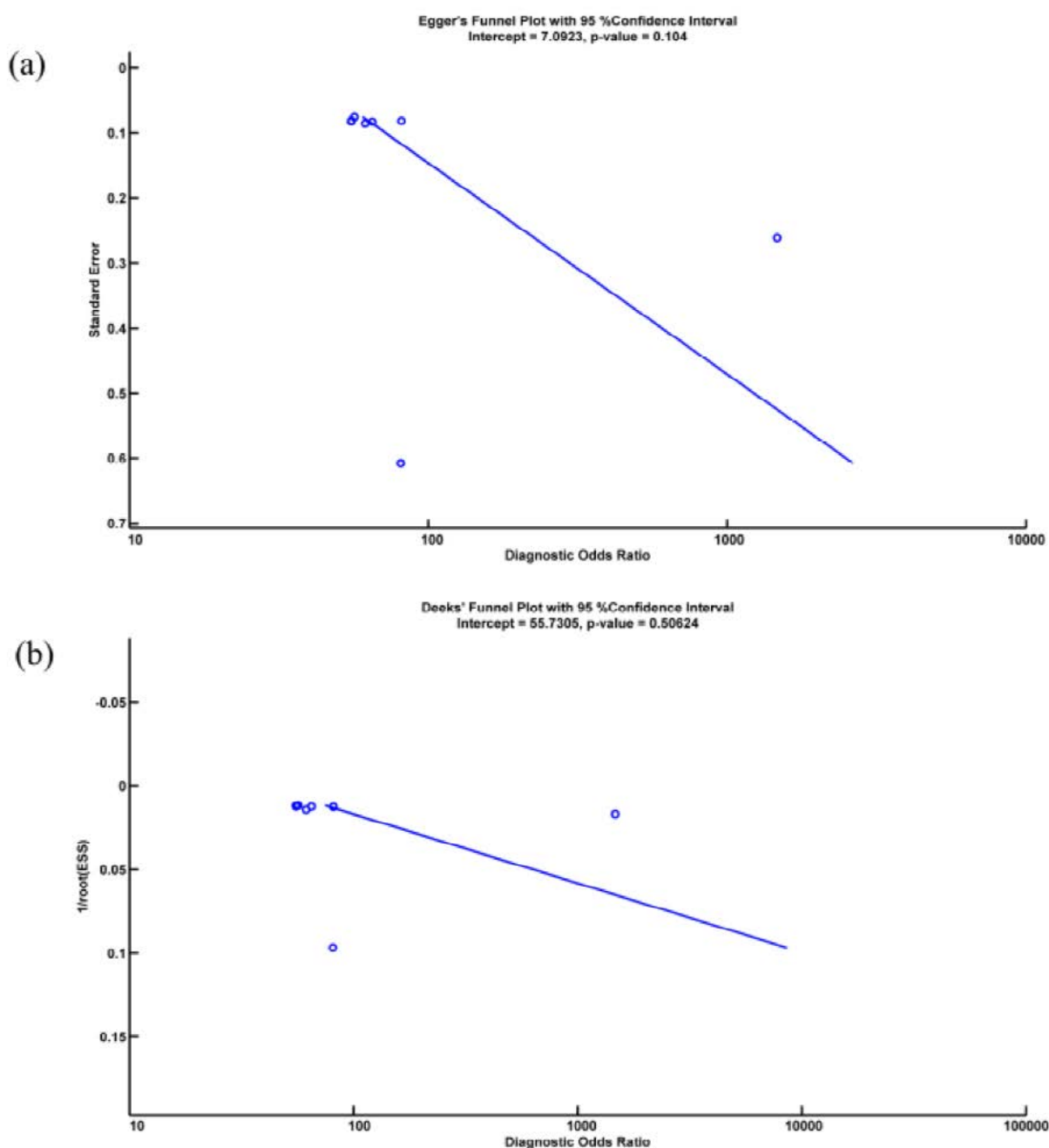
Figure 5. Publication bias test, (a) Egger's funnel plot (b) Deeks' funnel plot, (c) SVE funnel plot (d) SVT funnel plot, and (e) trim and fill assessment approach.
