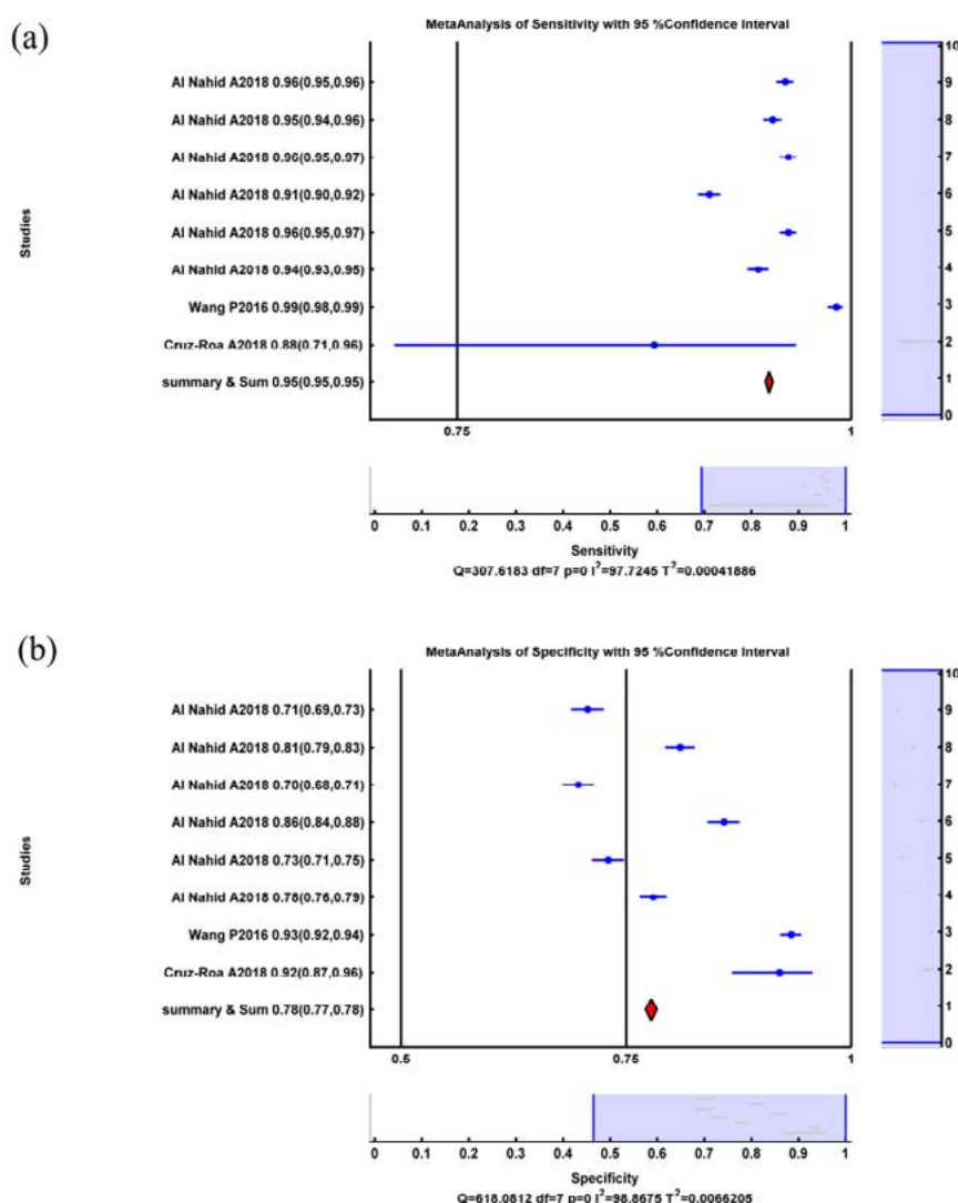
Figure 2. The meta-analysis forest plots of (a) sensitivity and (b) specificity with 95% confidence interval.
