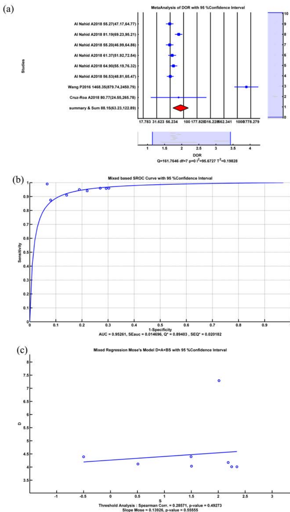
Figure 4. (a) Forest plot of diagnostic odds ratio of artificial intelligence systems in diagnosis of breast cancer (b) SROC of artificial intelligence systems in diagnosis of breast cancer, and (c) threshold analysis of eight artificial intelligence systems in diagnosis of breast cancer.
